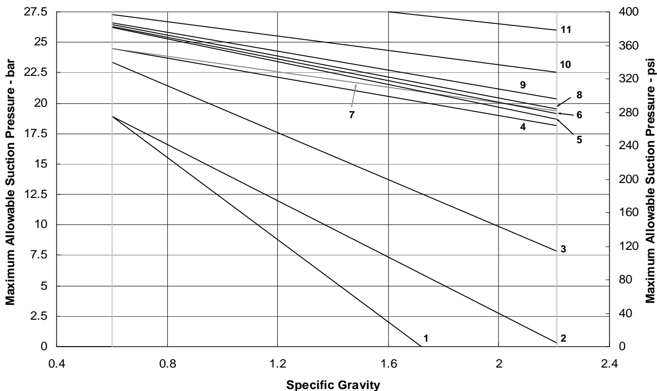
Figure 3-6B: Suction pressure limits 3500 r/min
